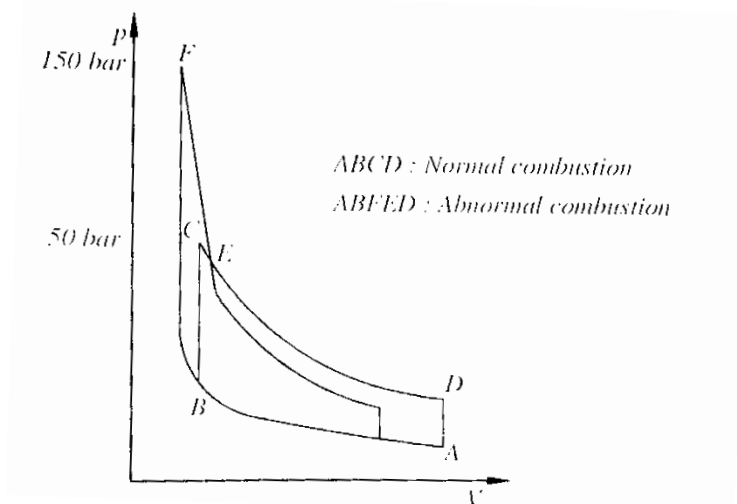
Fig.7. 10 Pressure rise due to knocking
