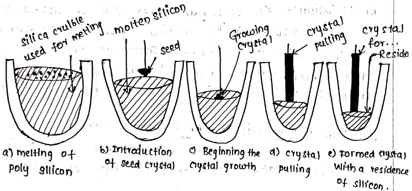
Czochralski process.
