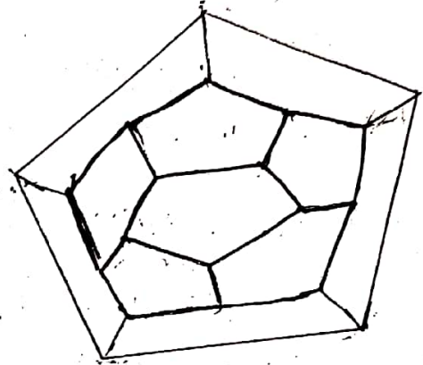
C_{20} fullerene
