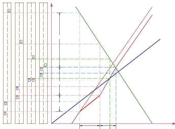
Figure 13:1: Time-space diagram: Illustration of overtaking sight distance
